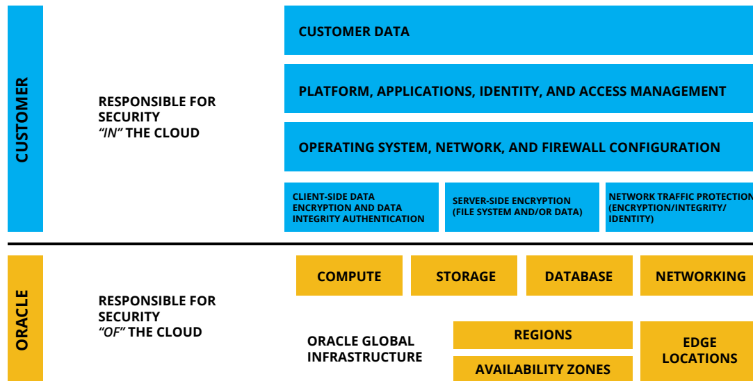
Figure 1. Oracle Cloud Infrastructure Classic and Platform Cloud Services Security .
