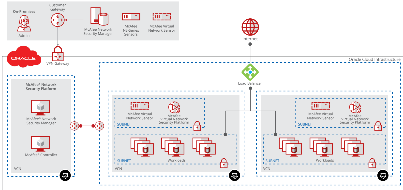
Figure 2. McAfee Virtual Network Security Platform protects north-south and east-west traffic in Oracle.
